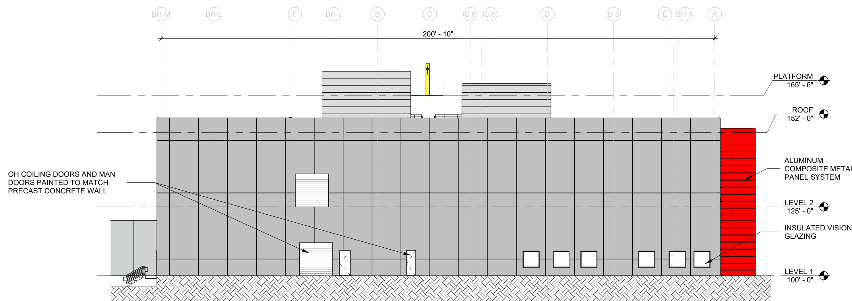
2 ELEVATION - SOUTH 1" = 20'-0"
