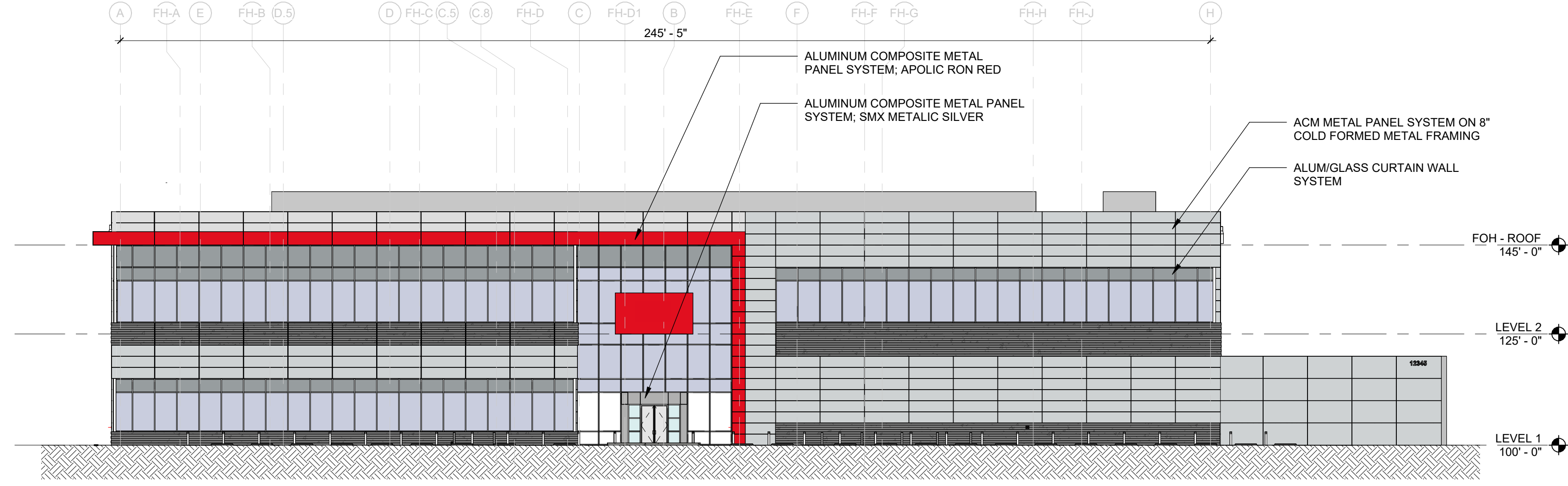
1 ELEVATION - NORTH 1" = 20'-0"
