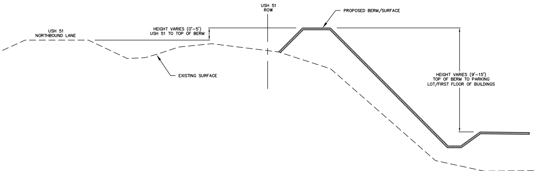
1 TYPICAL BERM CROSS SECTION 1 NOT TO SCALE (LOCATED ALONG THE HWY 51 RIGHT OF WAY)
